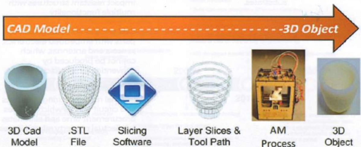
Generalized Additive Manufacturing process
